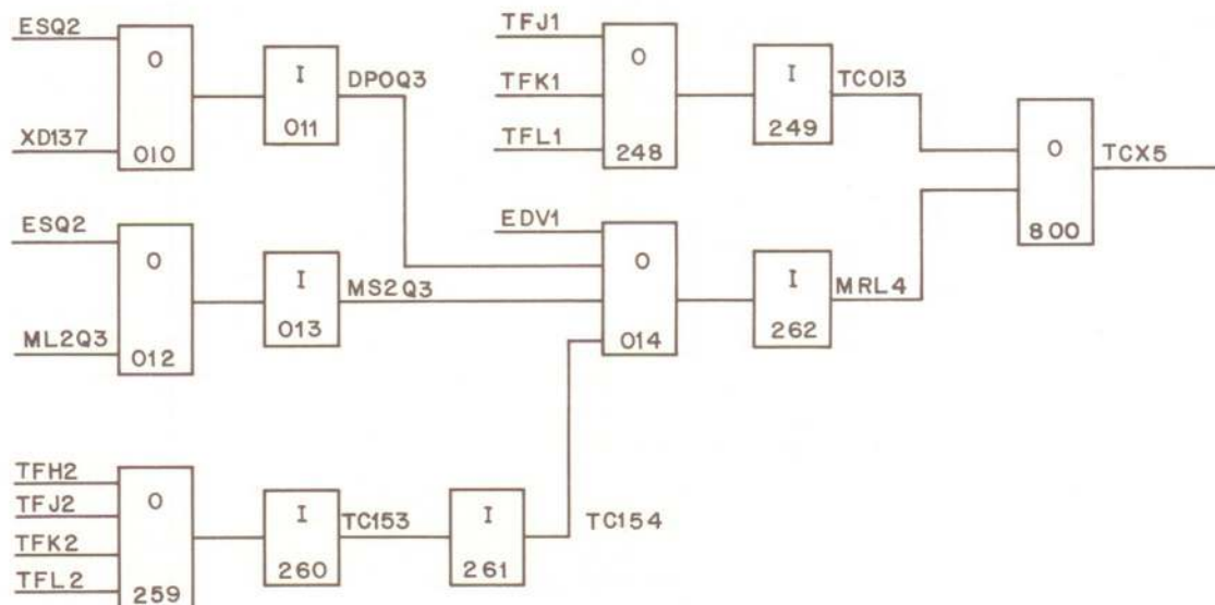
REGISTER EXPANSION LOGIC
