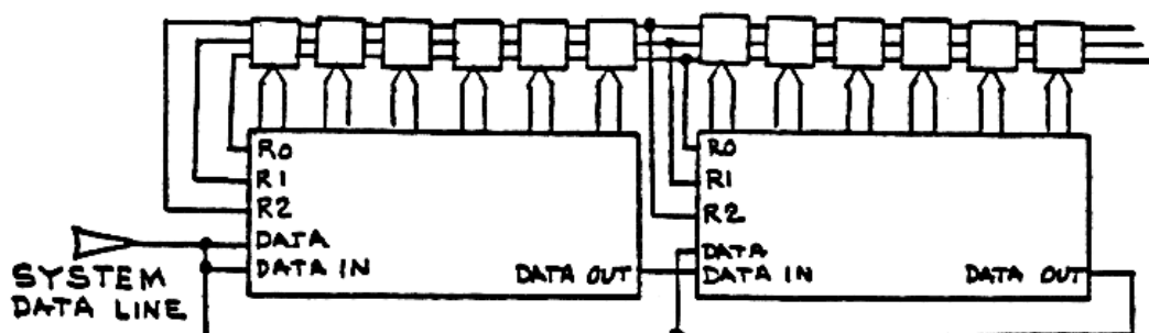
2 CHIP, 12 CHARACTER SYSTEM
