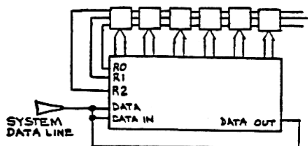
1 CHIP, 6 CHARACTER SYSTEM
