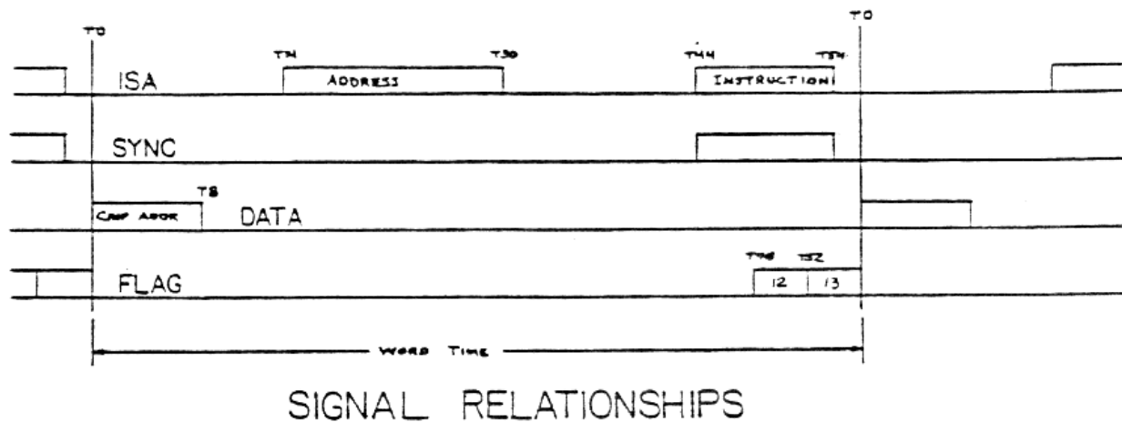
6.6 Figure 3: 41-C System Signals.
