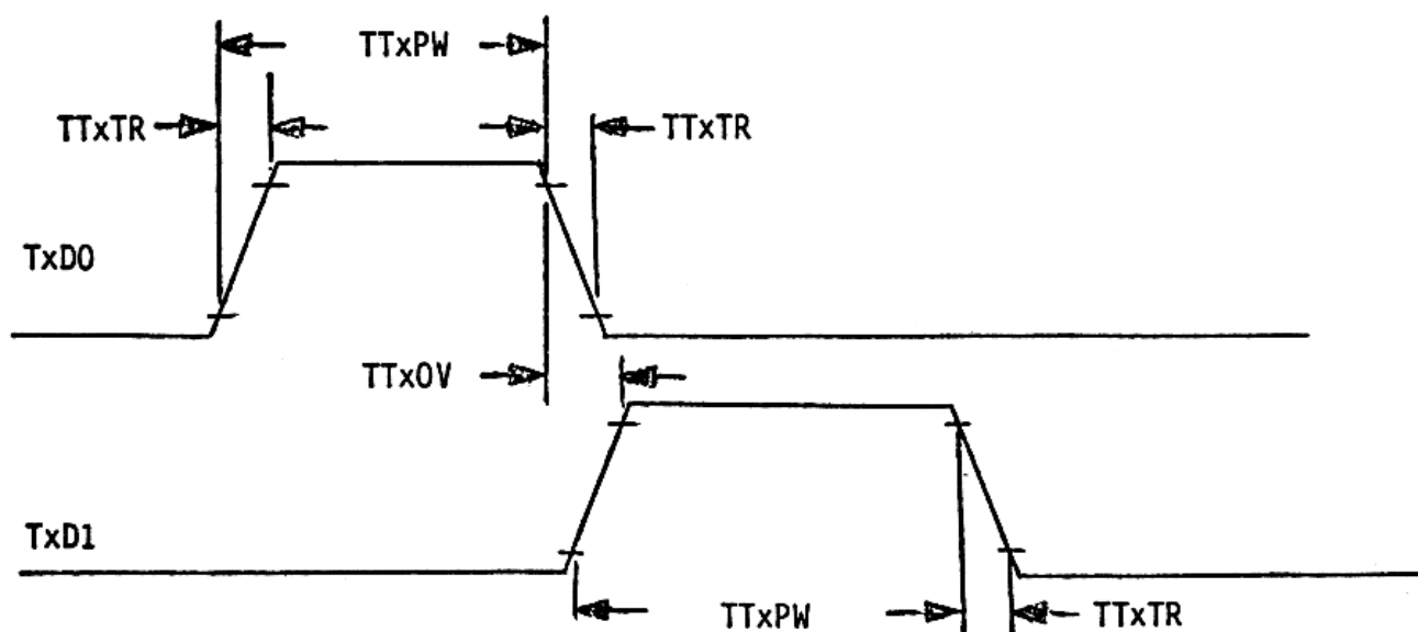
FIGURE 5 - PIL TRANSMITTER TIMING
