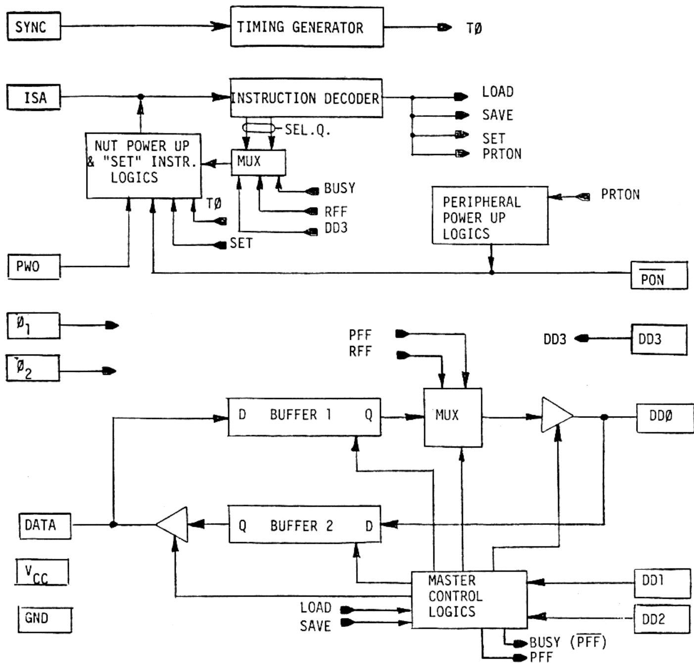
BLOCK DIAGRAM OF NUT PERIPHERAL INTERFACE CHIP
