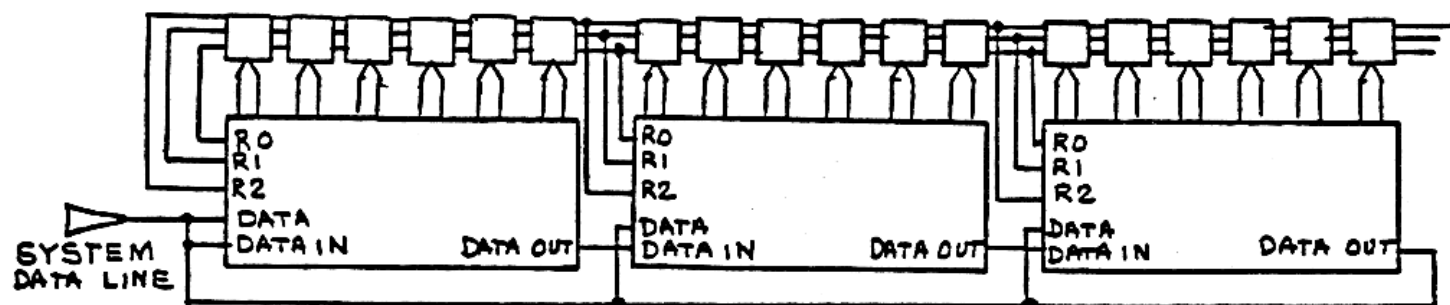
3 CHIP, 18 CHARACTER SYSTEM
