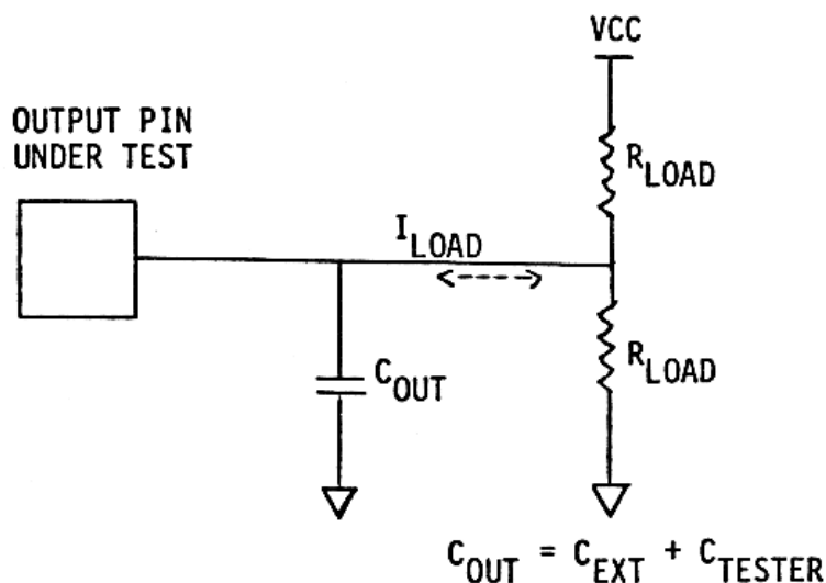
TEST CONDITION FOR OUTPUT PINS (Figure 4)
