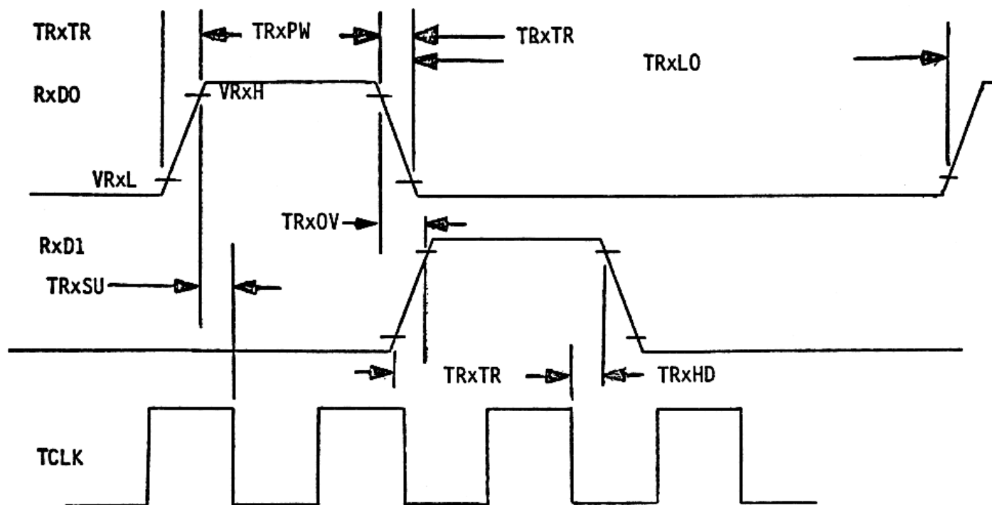
FIGURE 4 - PIL RECEIVER TIMING
