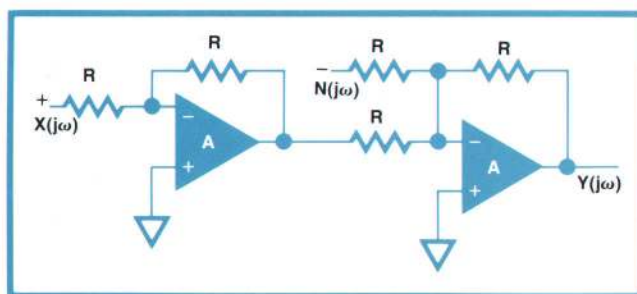
Fig. 2. An operational amplifier circuit for introducing noise N(j\omega) into a system without disturbing the system.
