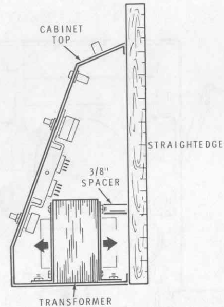
Detail 3-6A
