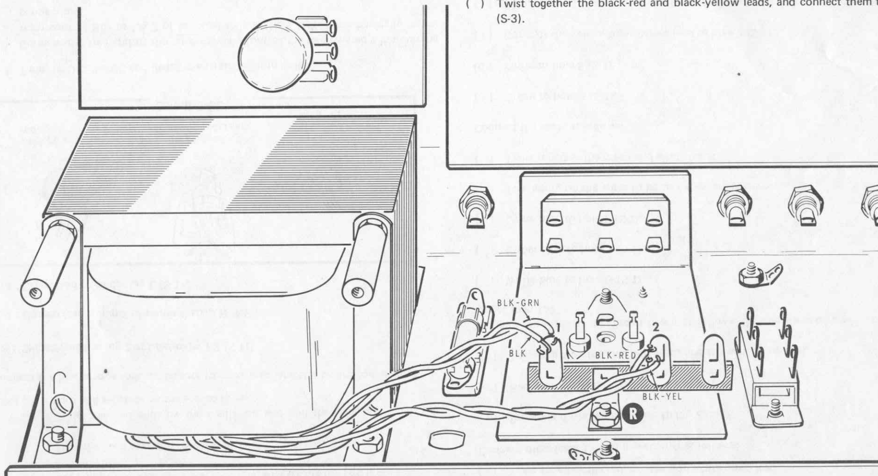
Detail 3-9A
