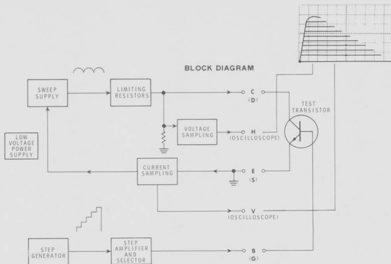
BLOCK DIAGRAM
