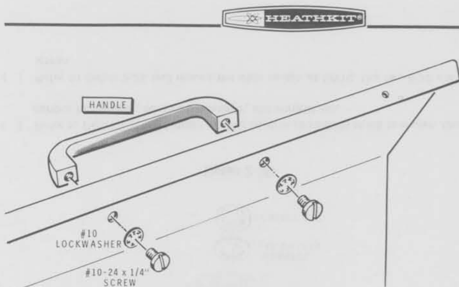
Detail 2-3G
