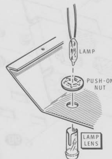
Detail 2-3F
