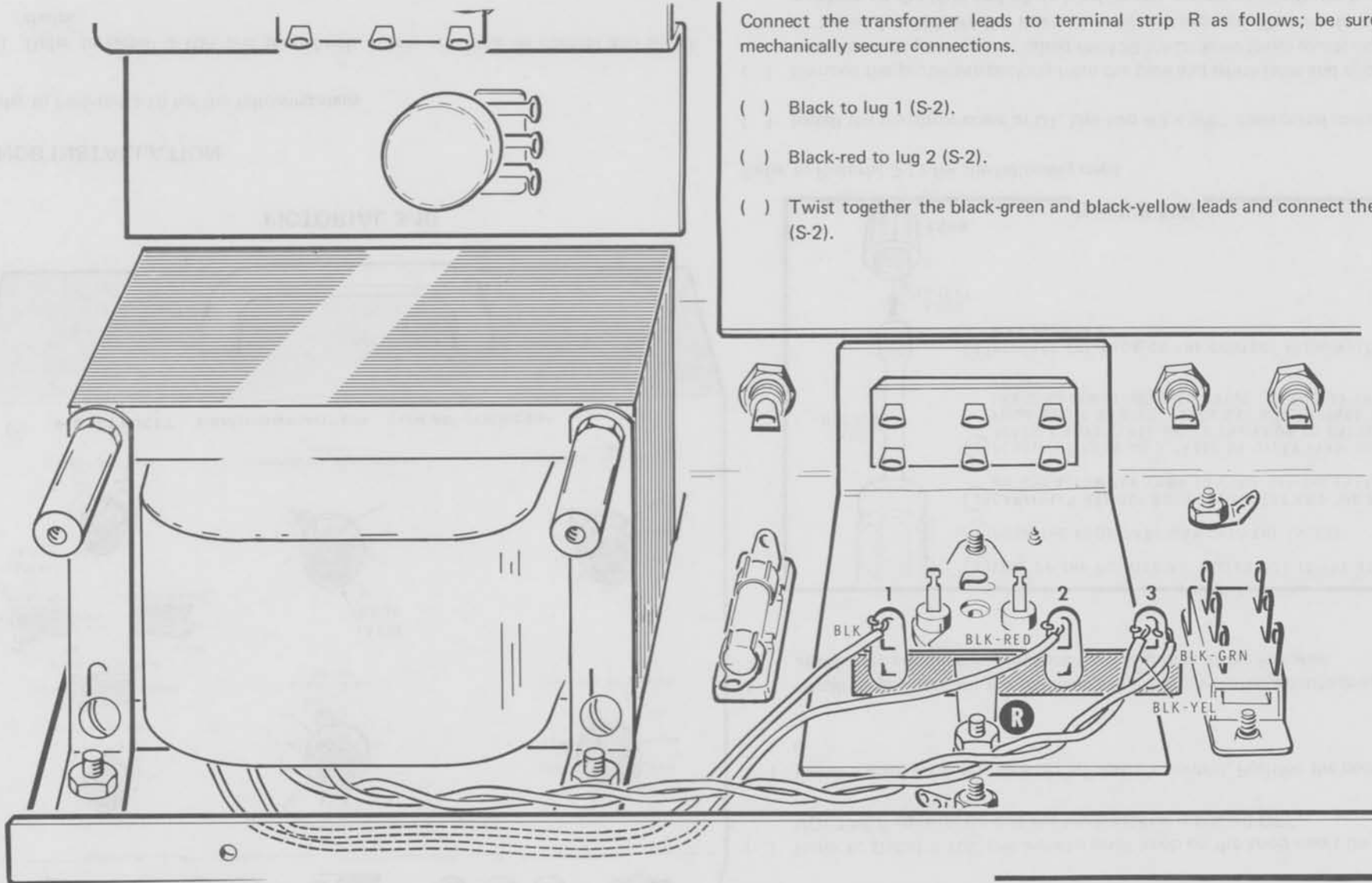
Detail 3-9B
