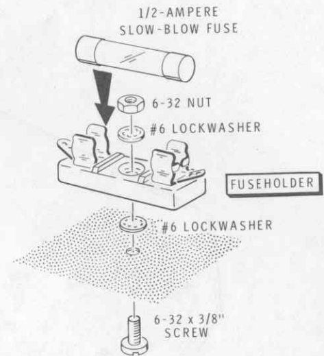
Detail 3-6B
