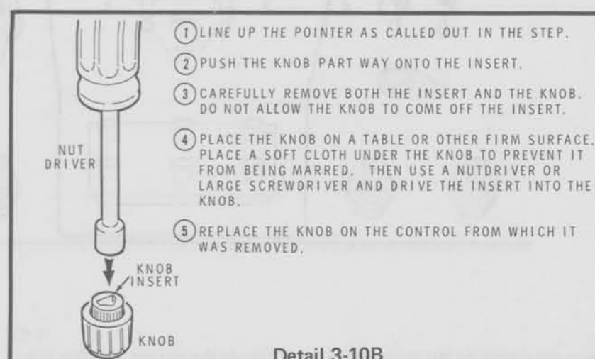
Detail 3-10B
