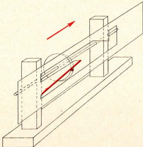
a) Grande came (F).
