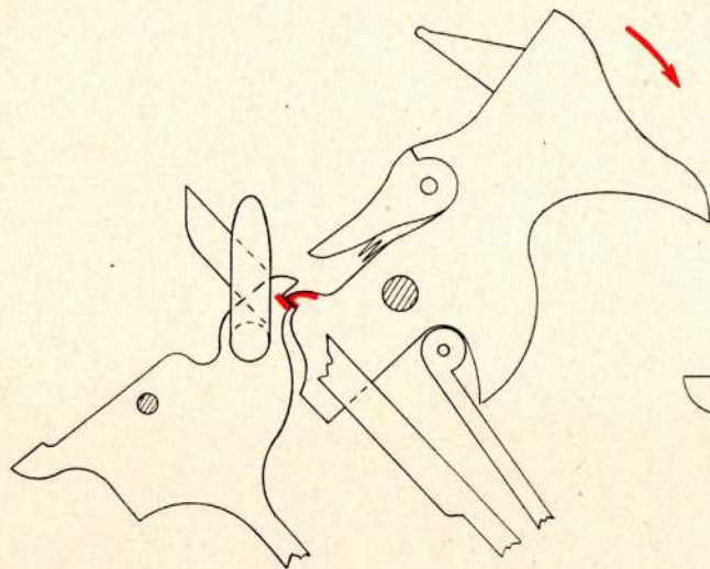
ARMÉ (Tir intermittent).
