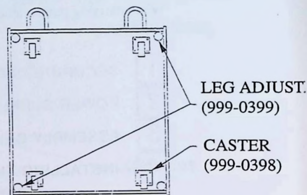
FIG. 6.1 BOTTOM VIEW
