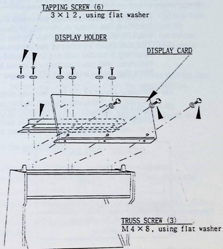
FIG. 6.4 INSTALLING THE DISPLAY CARD
