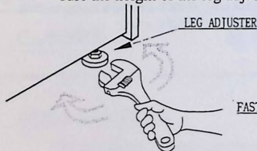
FIG. 6.2 LEG ADJUSTER
