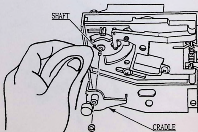
FIG. 10. 2 CLEANING THE COIN SELECTOR
