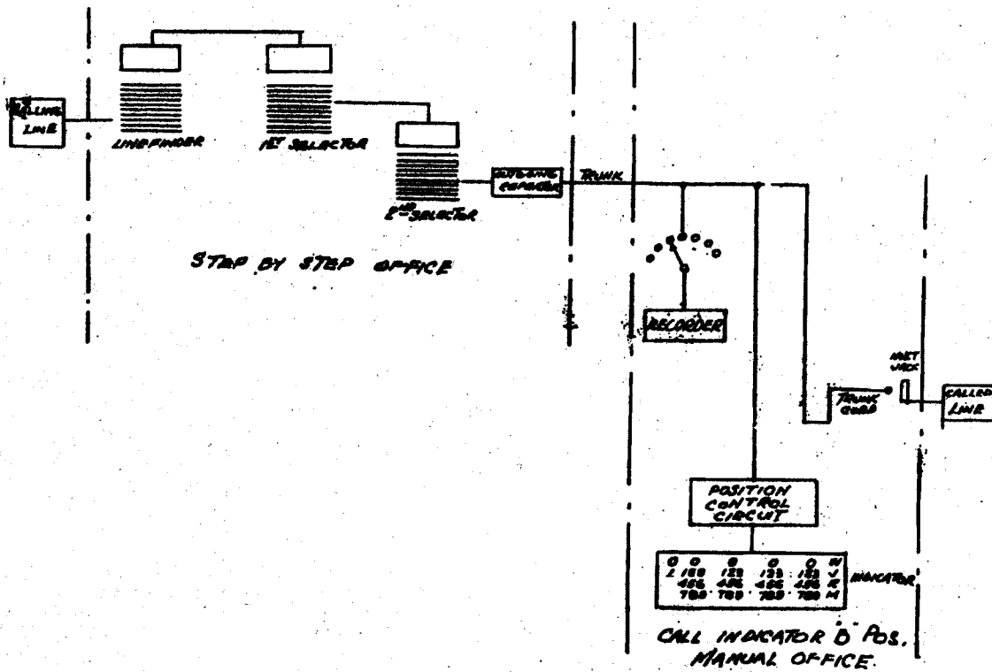
FIG. 24 "STEP-BY-STEP CALL INDICATOR"
