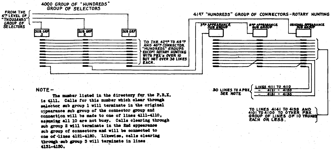
FIG. 23 "MULTIPLE SLIP ARRANGEMENT FOR CONNECTOR GROUPS SERVING PBX GROUPS OVER 10 TERMINALS
