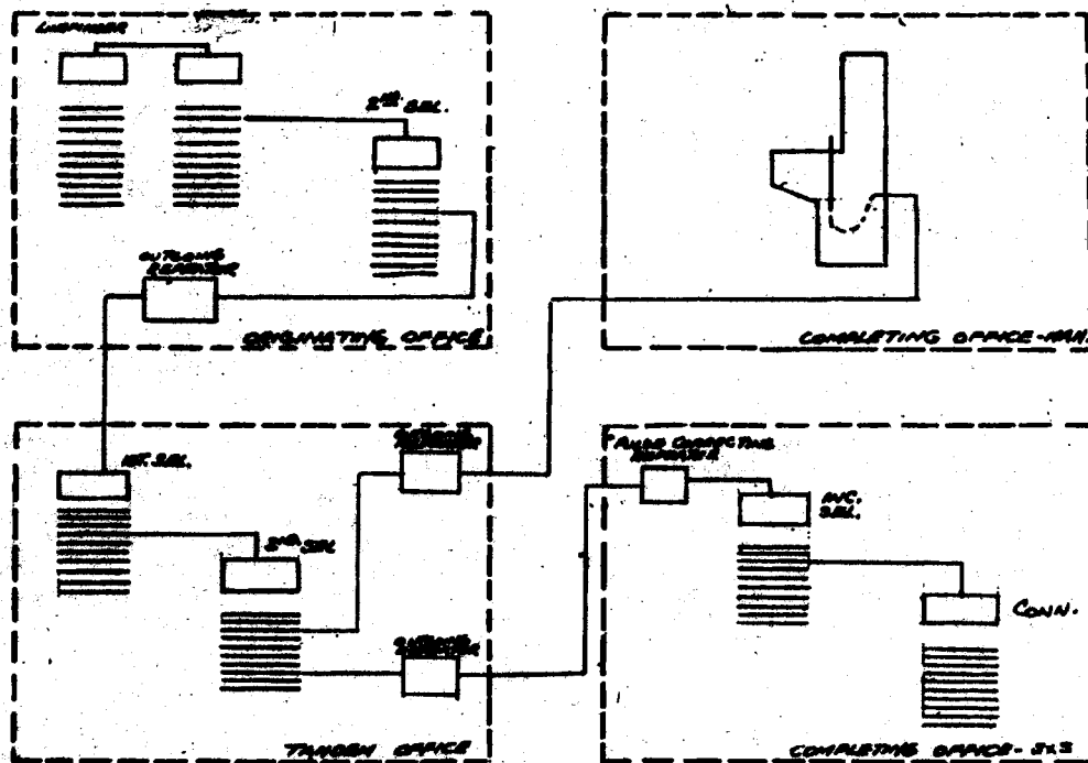
FIG. 25 "TANDEM OPERATION"
