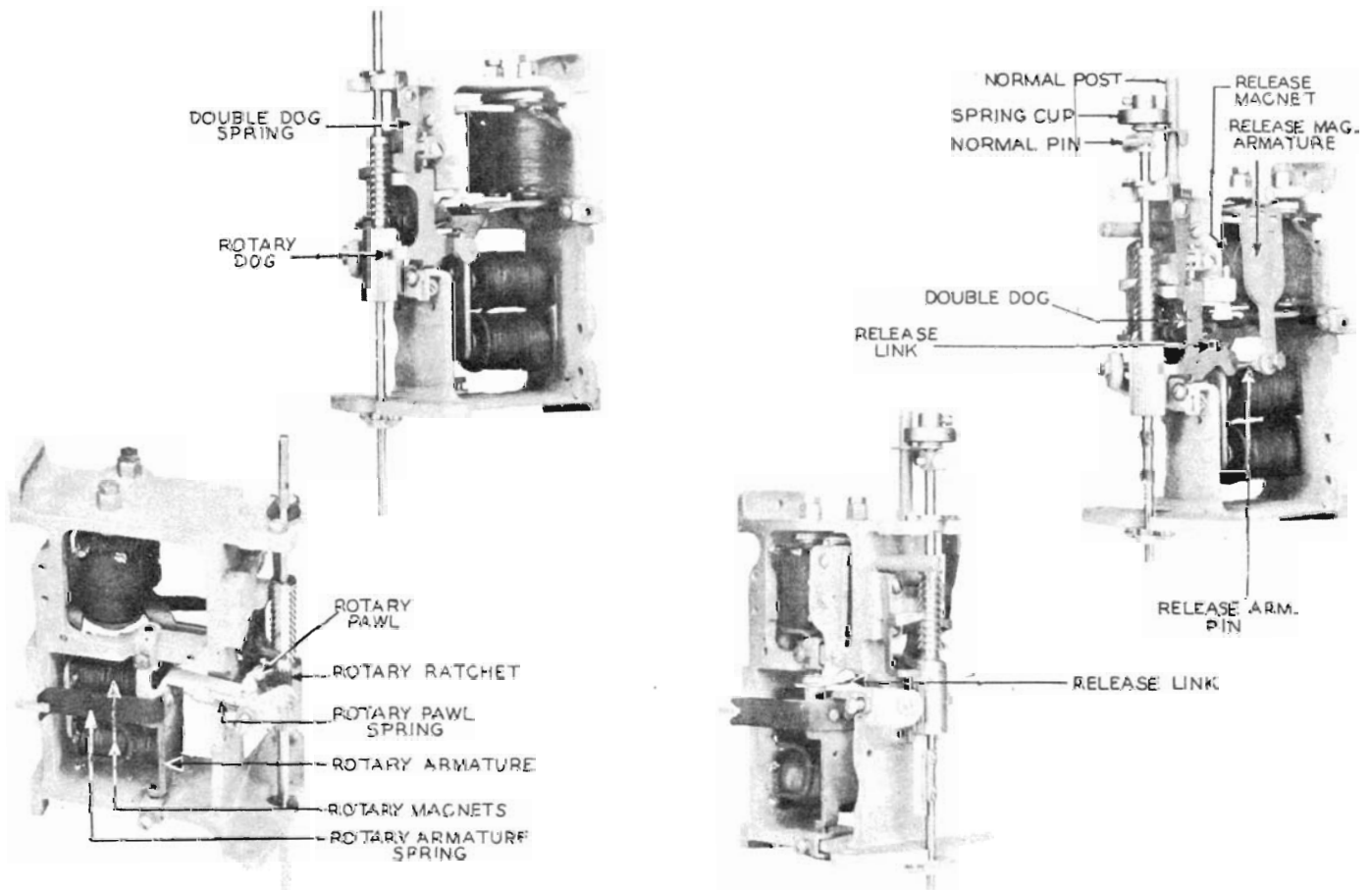
FIG. 9 ROTARY STEPPING MECHANISM
