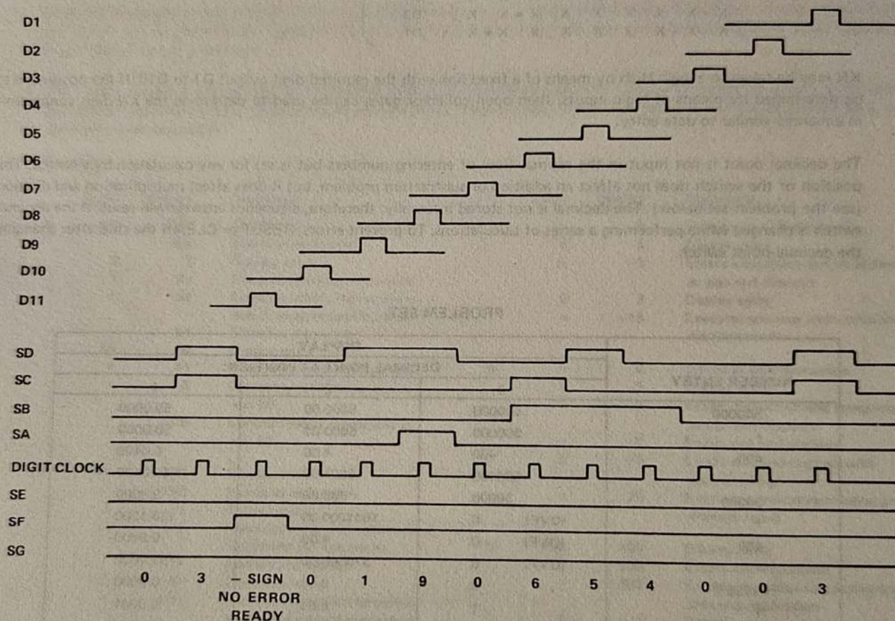
DATA OUTPUT TIMING EXAMPLE
