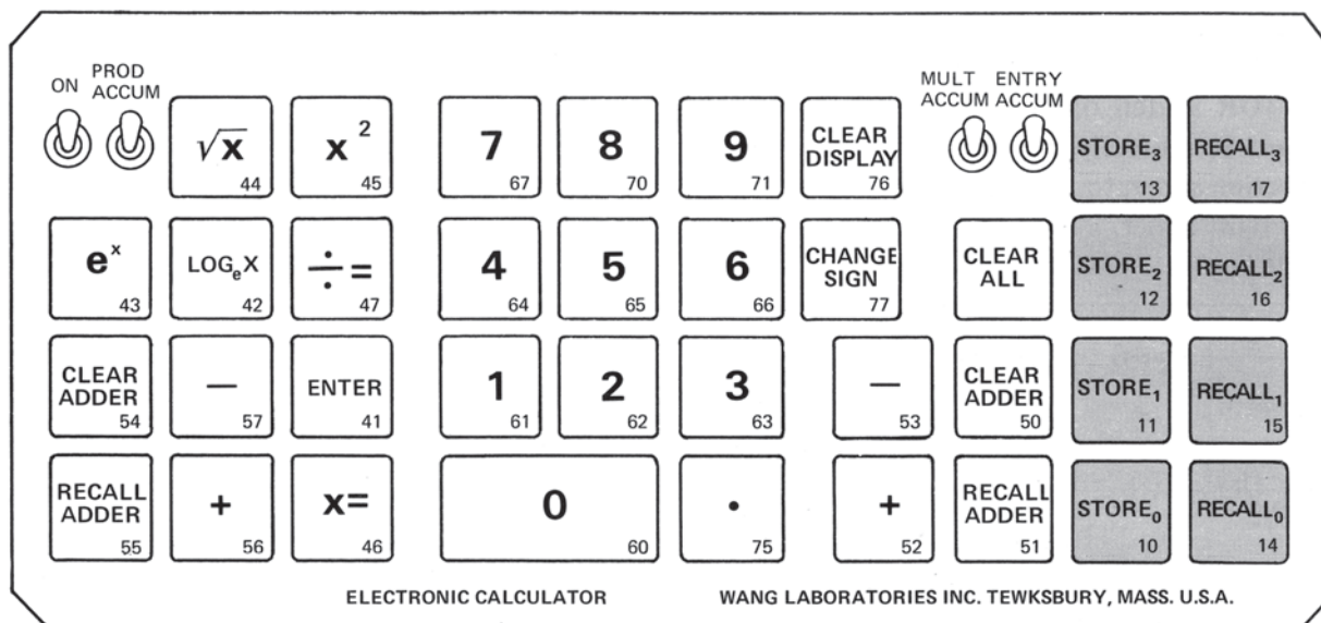
Figure 3-12. Model 360 Storage Register Keys.
