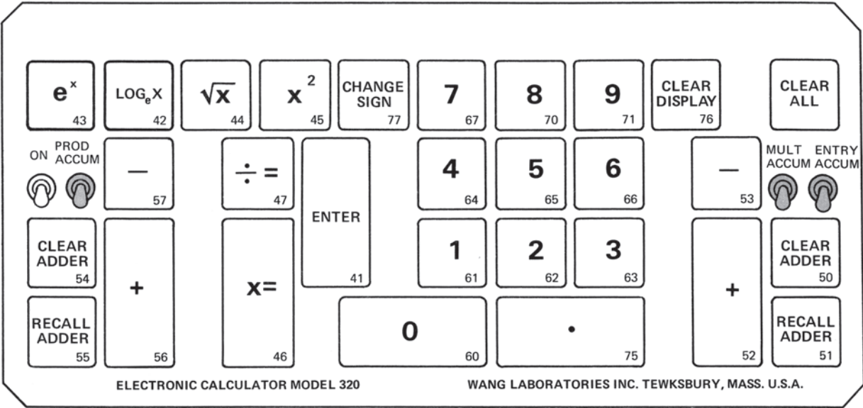
Figure 3-11. Accumulator Switches.
