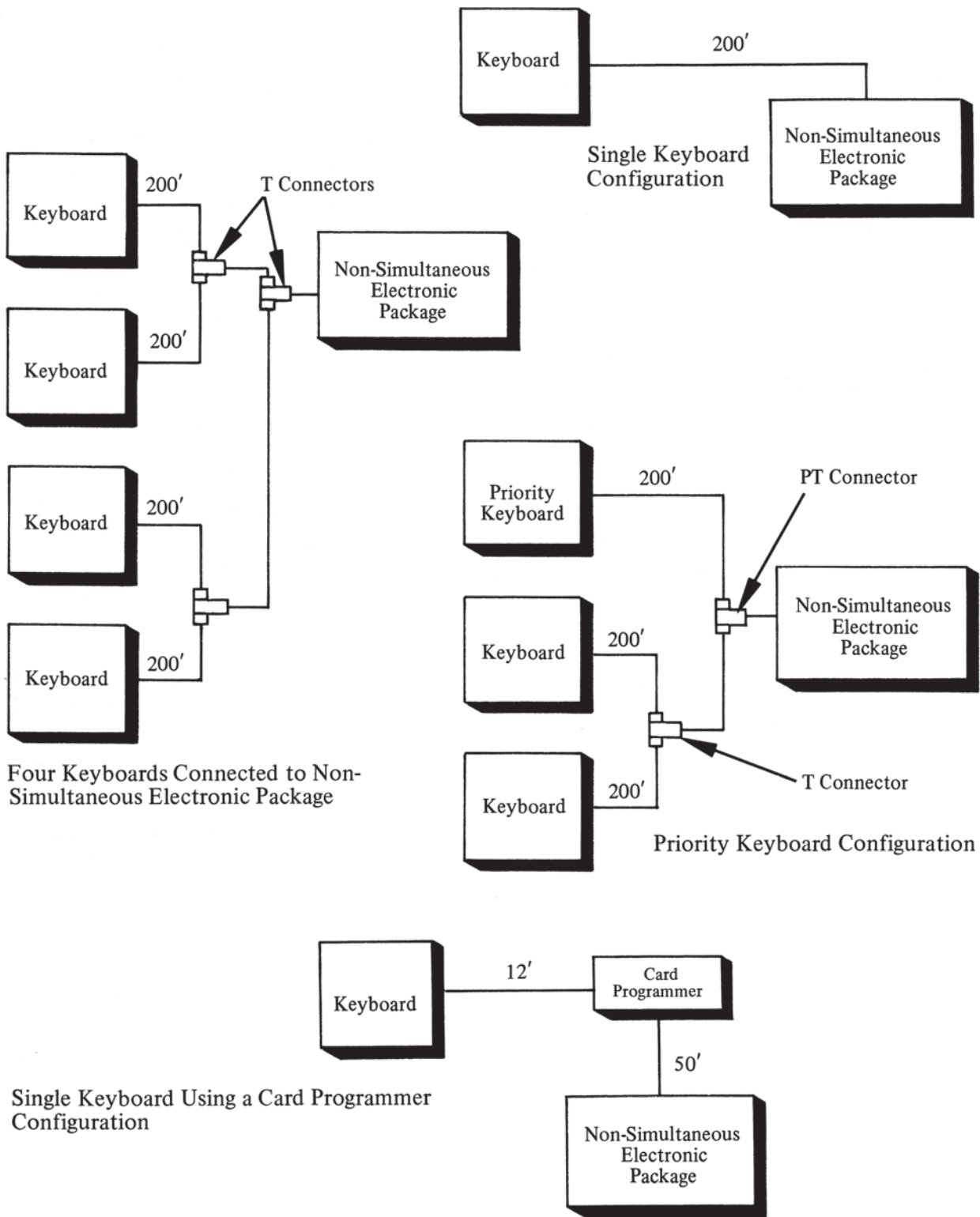
Figure 2-1. Interconnecting Arrangements
