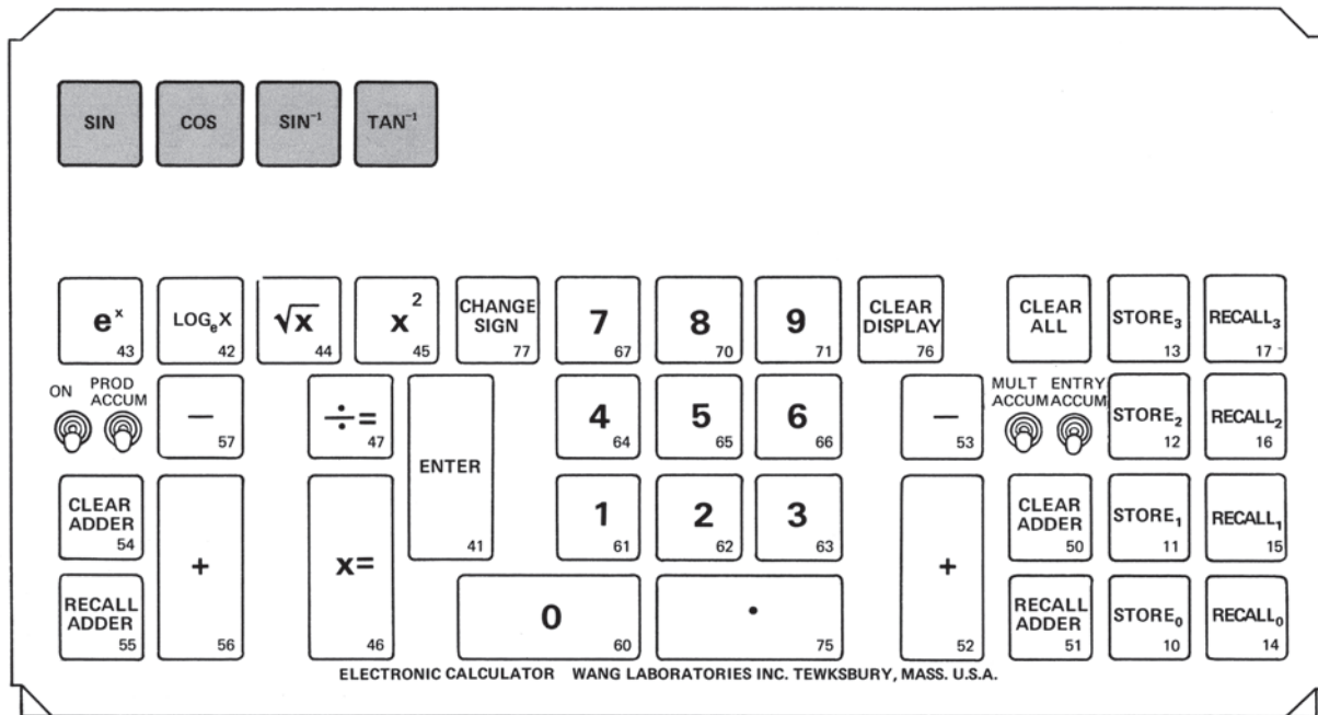
Figure 3-15. Trigonometric Keys.
