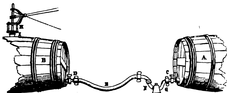
HILTON'S INSTRUMENT.
