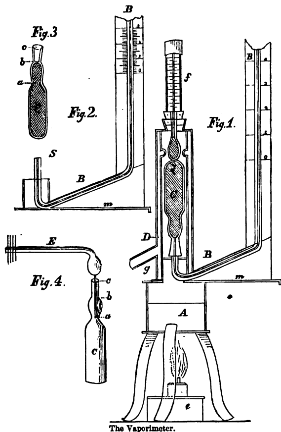
The Vaporimeter.
